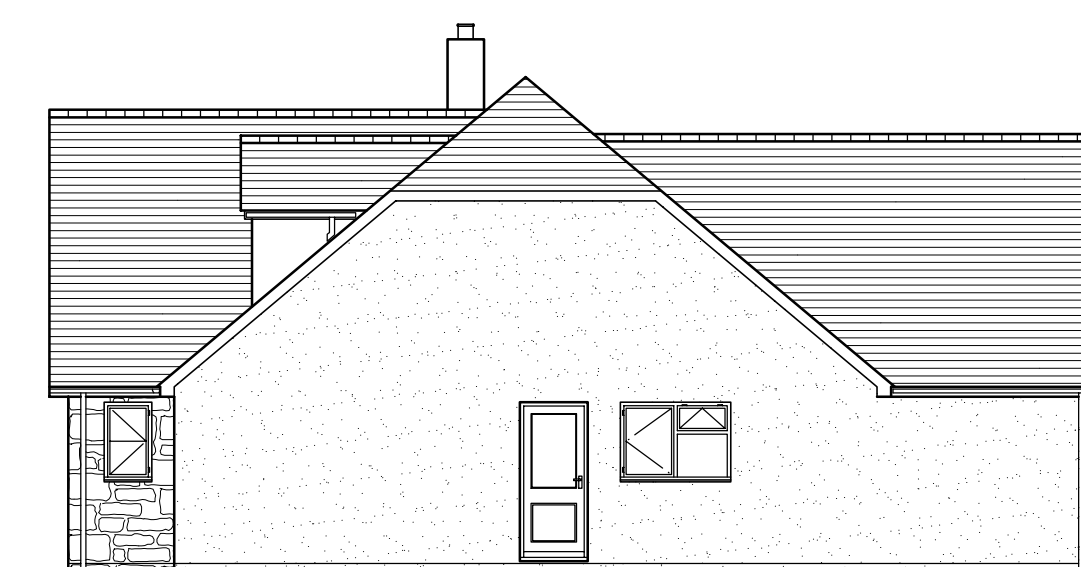
SIDE ELEVATION - NORTH EAST
