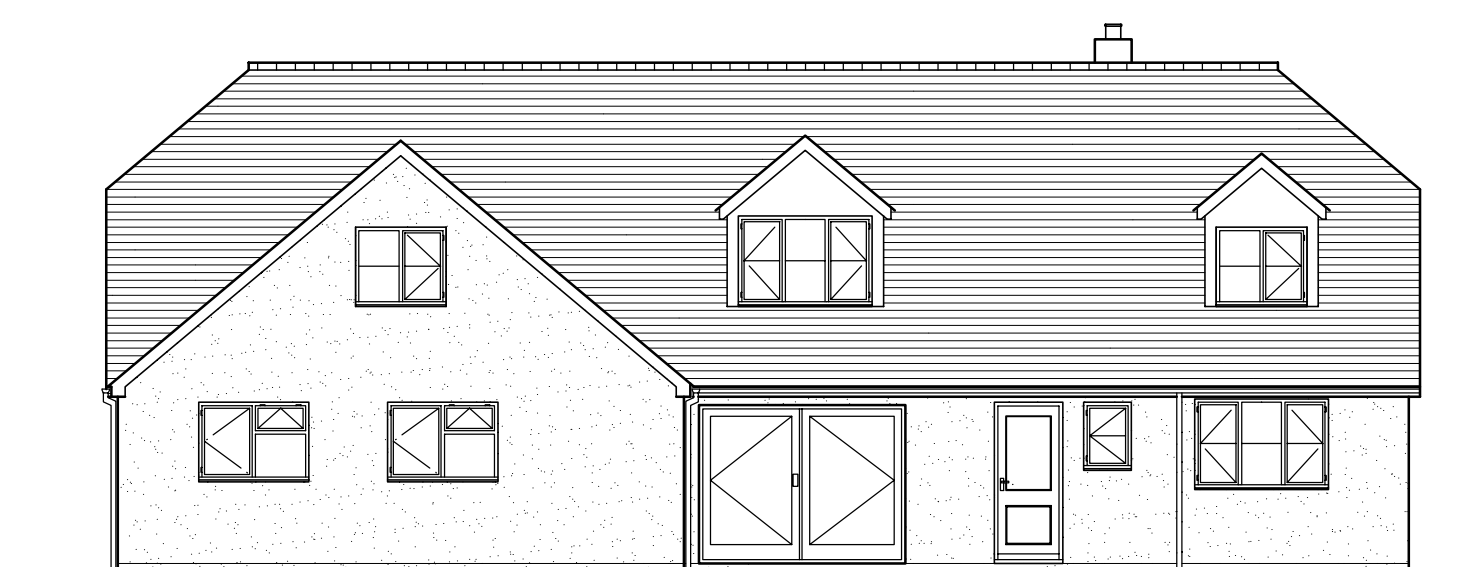
REAR ELEVATION - NORTH WEST
